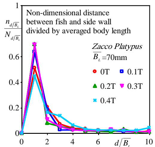
Figure 4(b). Magnet area Figure 4. Frequency distribution of d/\bar{B}_L
